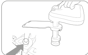
Pushing the button (protrusion) of the Foot Plate hole inside, join the Foot Plate and the Height Control Bar
